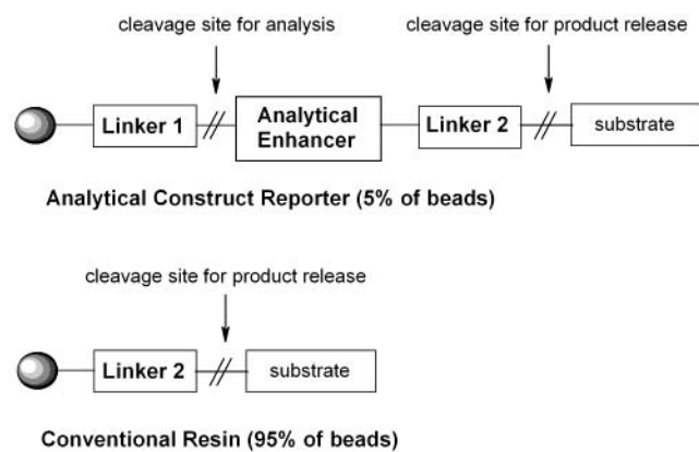
Figure 1. The principle of the “reporter resin”. Introduction of an analytical enhancer between the linker used in the solid-phase synthesis (linker 2) and another chemically orthogonal linker (linker 1) in 5% of the beads enables monitoring of each chemical step by cleavage of linker 1 followed by LC/MS analysis.
