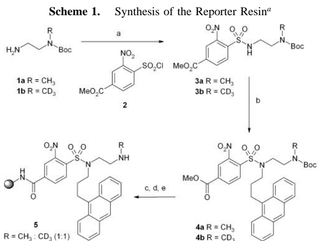
Figure 1. The principle of the “reporter resin”. Introduction of an analytical enhancer between the linker used in the solid-phase synthesis (linker 2) and another chemically orthogonal linker (linker 1) in 5% of the beads enables monitoring of each chemical step by cleavage of linker 1 followed by LC/MS analysis.
